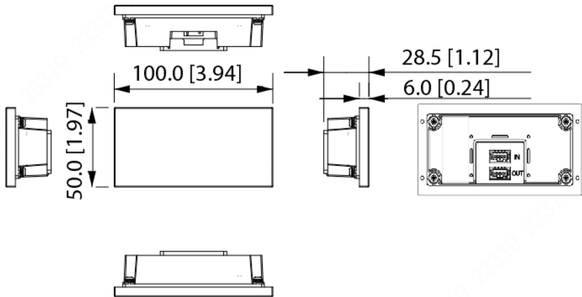
Figure 2-1 Dimensions (unit: mm [inch])
